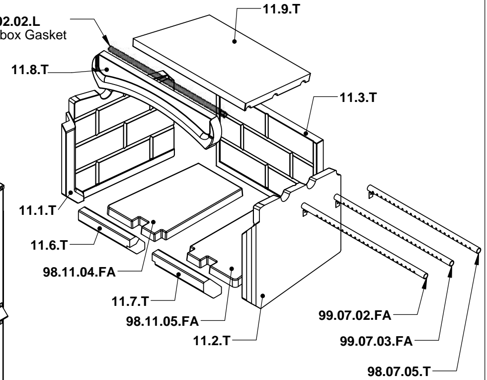
99.11.01.L Complete Refractory Brick Set
